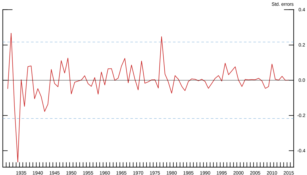
FIGURE 3 – Influential Observations
