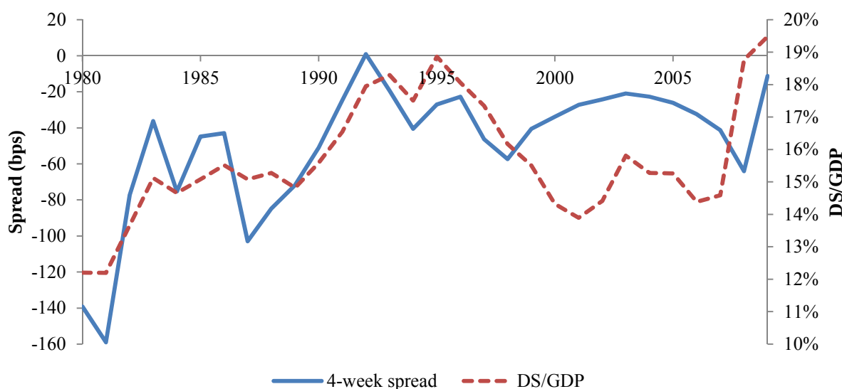
Panel B: 4-week T-bill premium (actual yield minus fitted yield) and the short-term debt-to-GDP ratio
